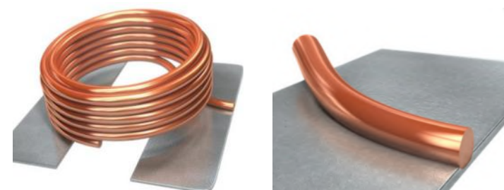
Figure 1 - The direct contact method of the WE-MXGI enables low R_{DC} values
