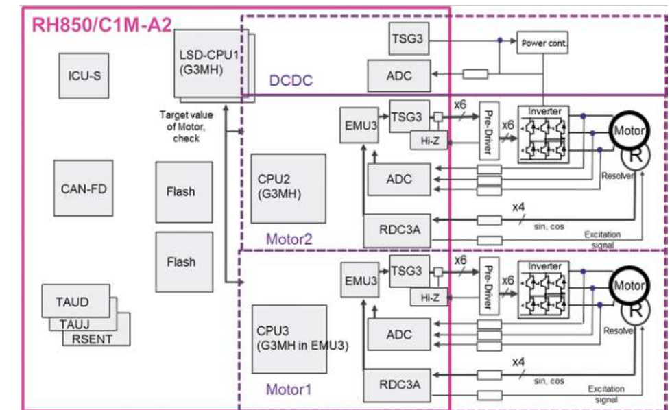
Figure 7: System example to control dual e-motor/generator
