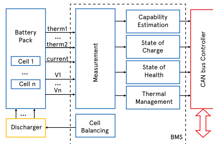
Figure 2: Functional block diagram of BMS
