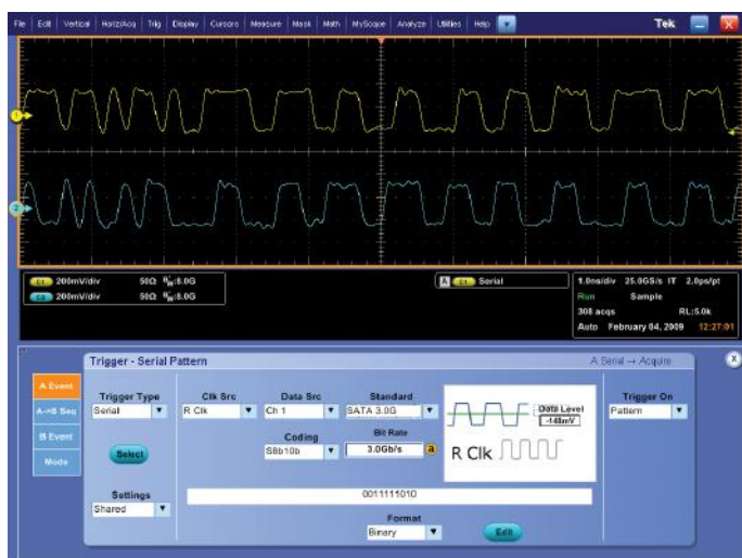
Figure 49. A DPO provides an ideal solution for non-repetitive, high-speed, multi-channel digital design applications.
