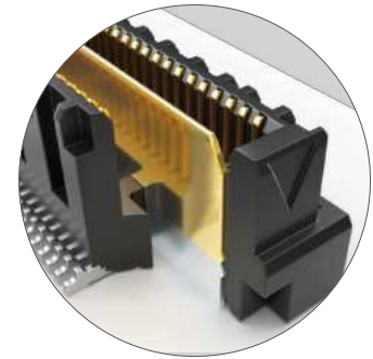
Integral ground plane improves electrical performance and reduces crosstalk
