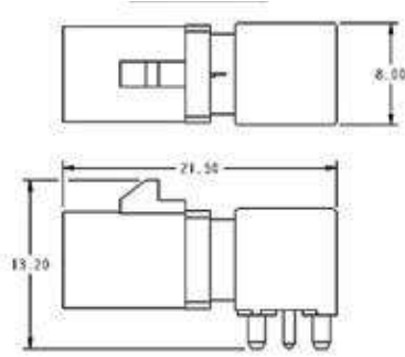
2FA1-NXRP-PCBB2
