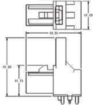
4FA1-NXRP-PCB-4
