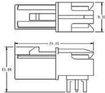
FA1-NXRP-PCB-6A
