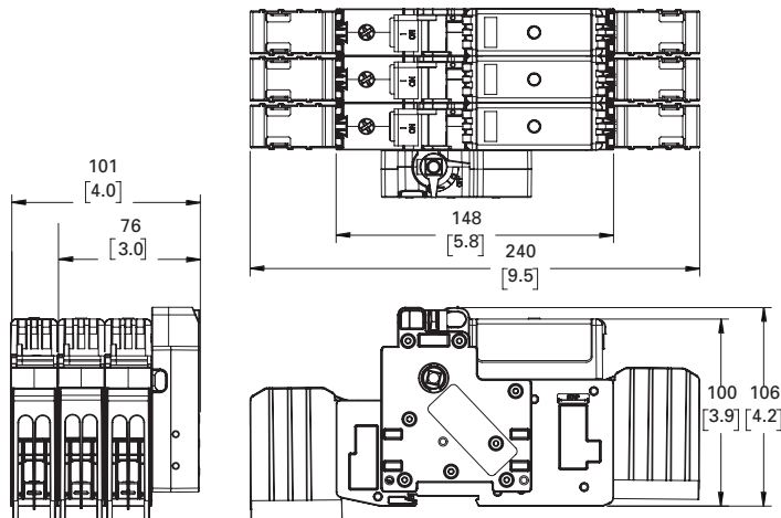
100 amp switches
